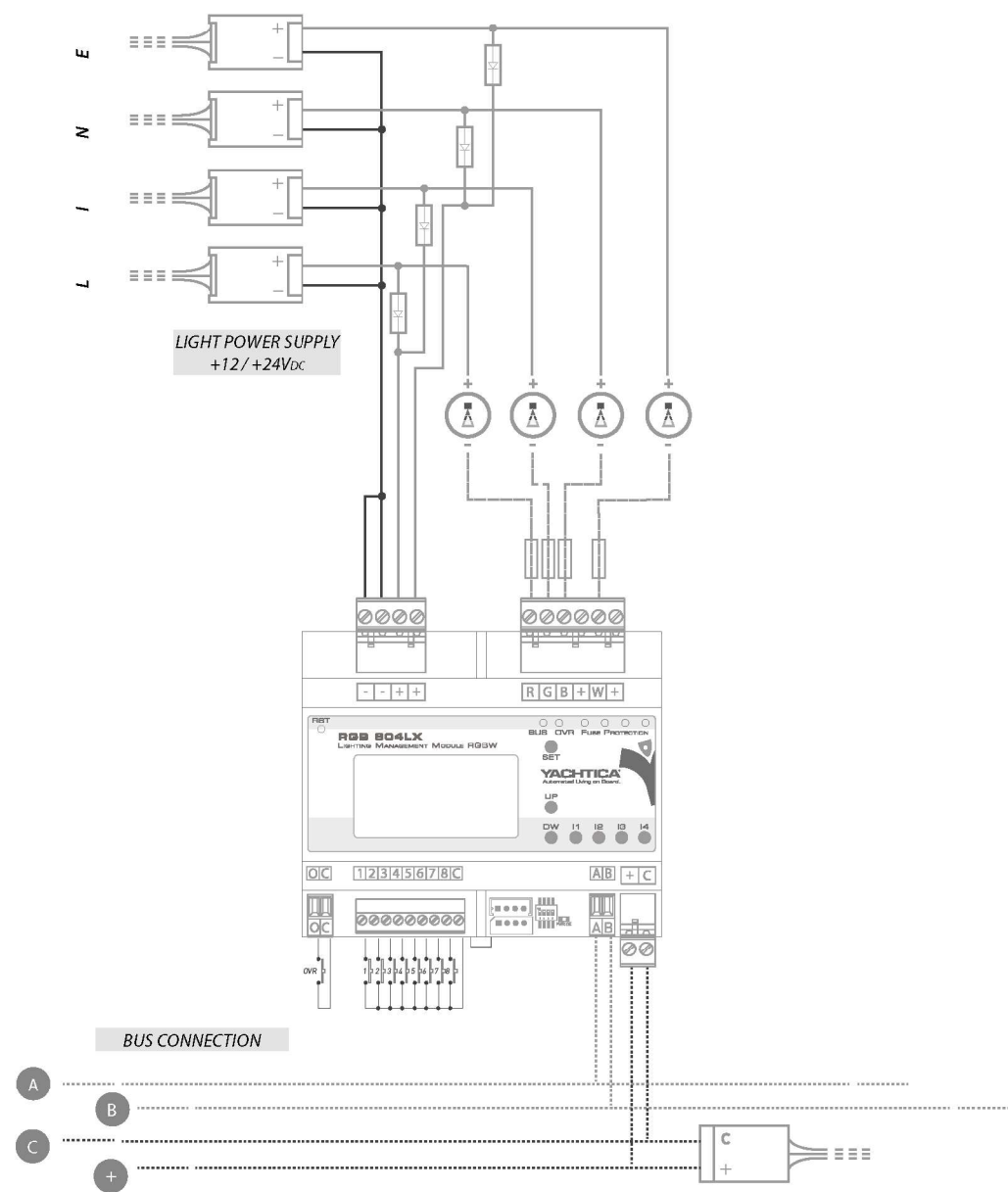
SCHEME 4: Wiring with direct positive (4 White)
